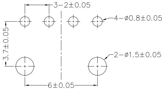
PCB Layout T=1.2mm
